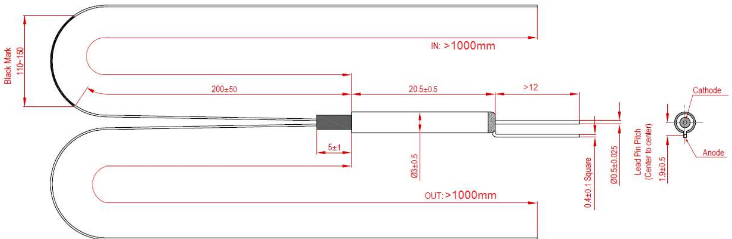
Figure 1. Compact Unidirectional Tap Photo Detector
