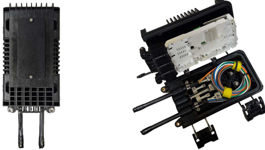
4-Port MMT closed and open views
